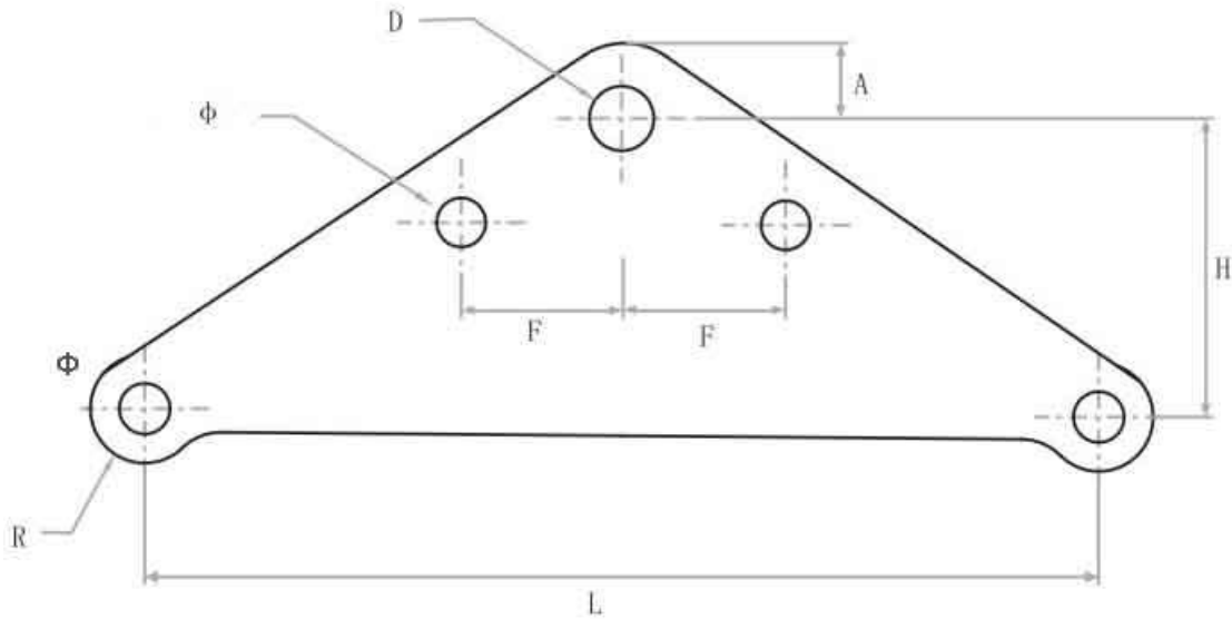
Yoke Plate
